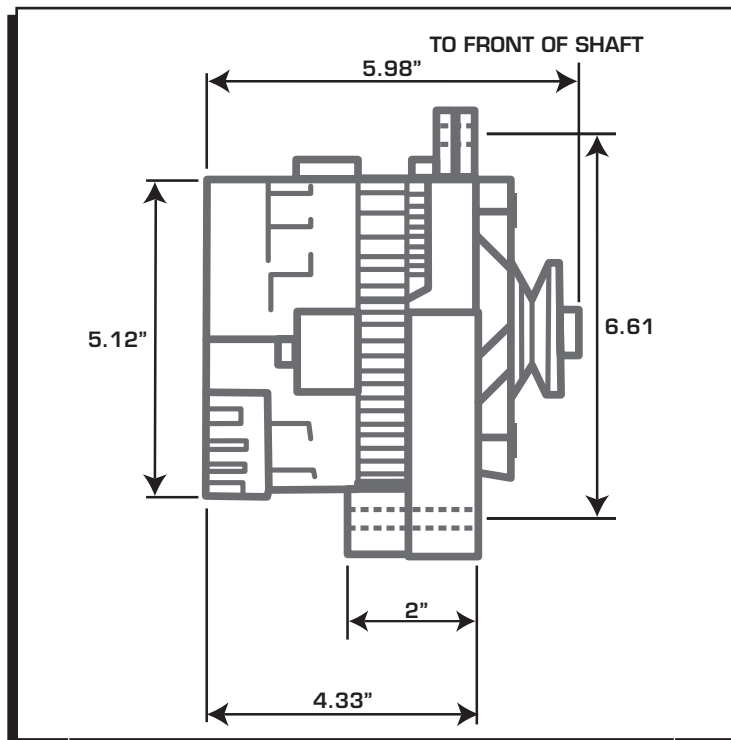
Figure 2 Alternator Dimensions.
