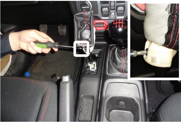
48. Install screw (removed step 7) to secure transfer case shifter to stem.
