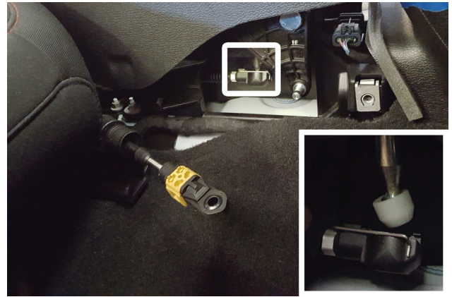
16. Disassemble lower cable from pivot cup, accessed on front passenger side of console.
